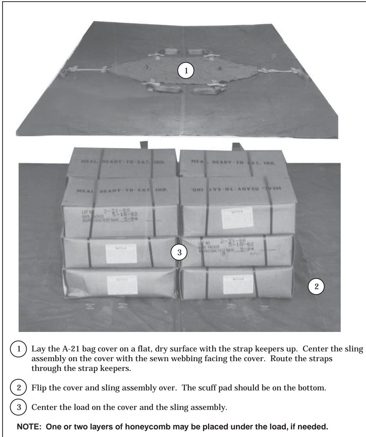
Figure 6-1. Container and Load Positoned
