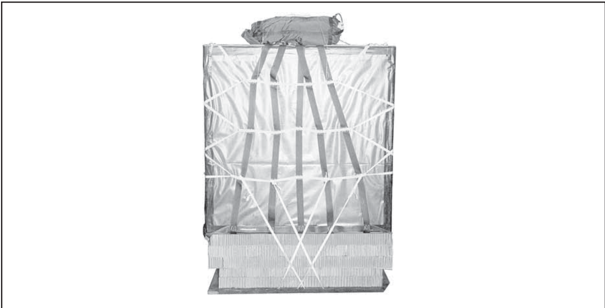
Figure 12-1. Fully Rigged LCADS for High-Velocity Airdrop
