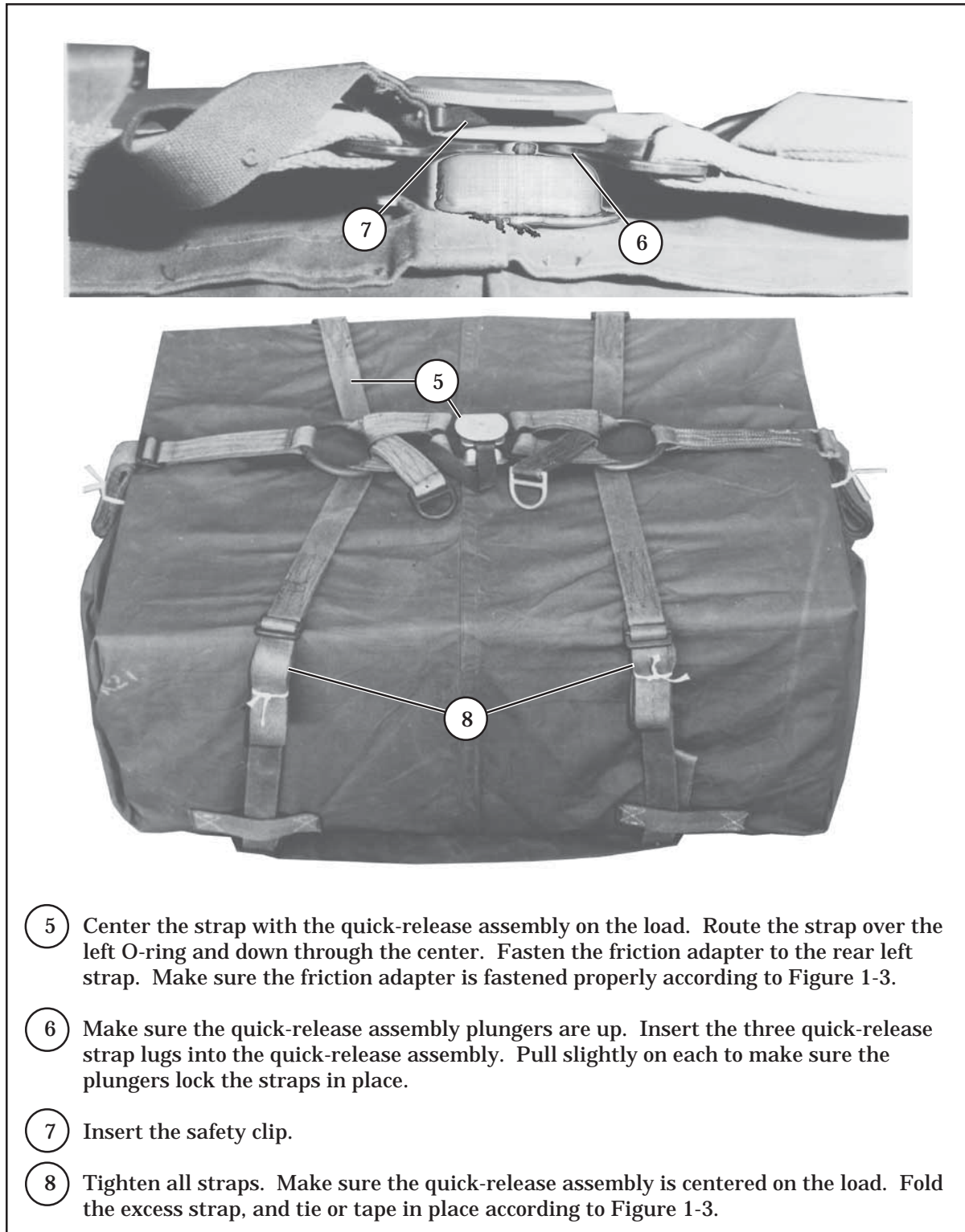
Figure 6-2. Container Rigged (Continued)
