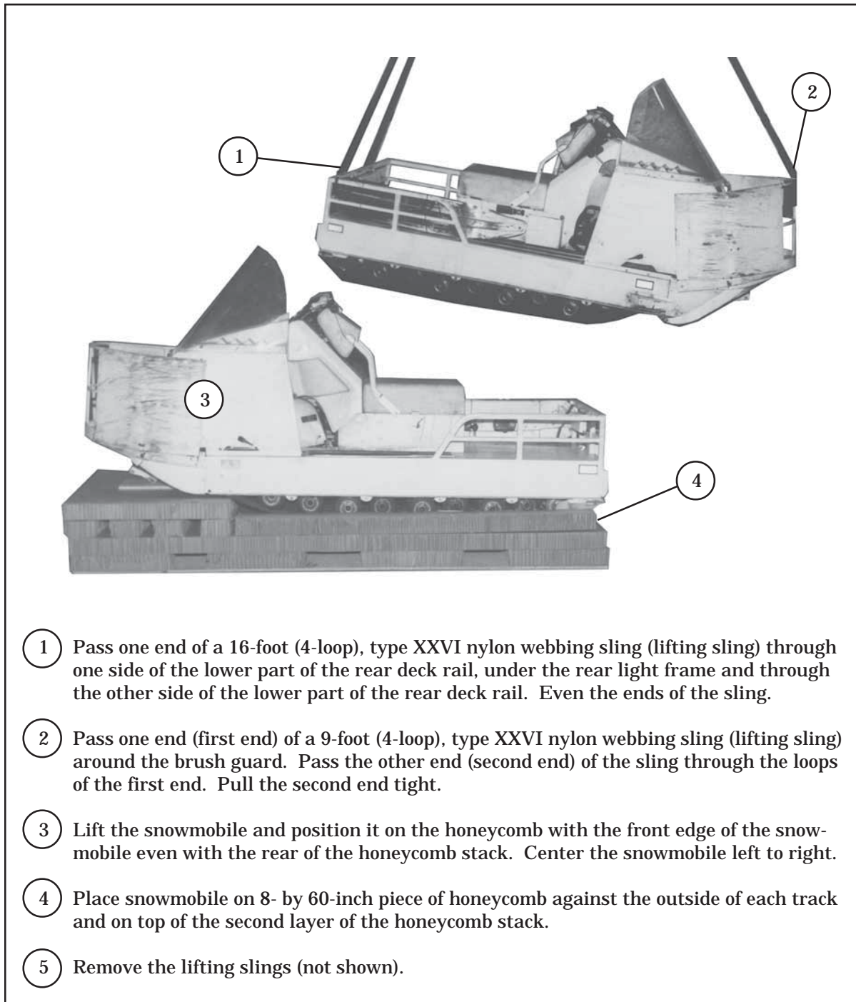
Figure 11-3. Snowmobile Positioned
