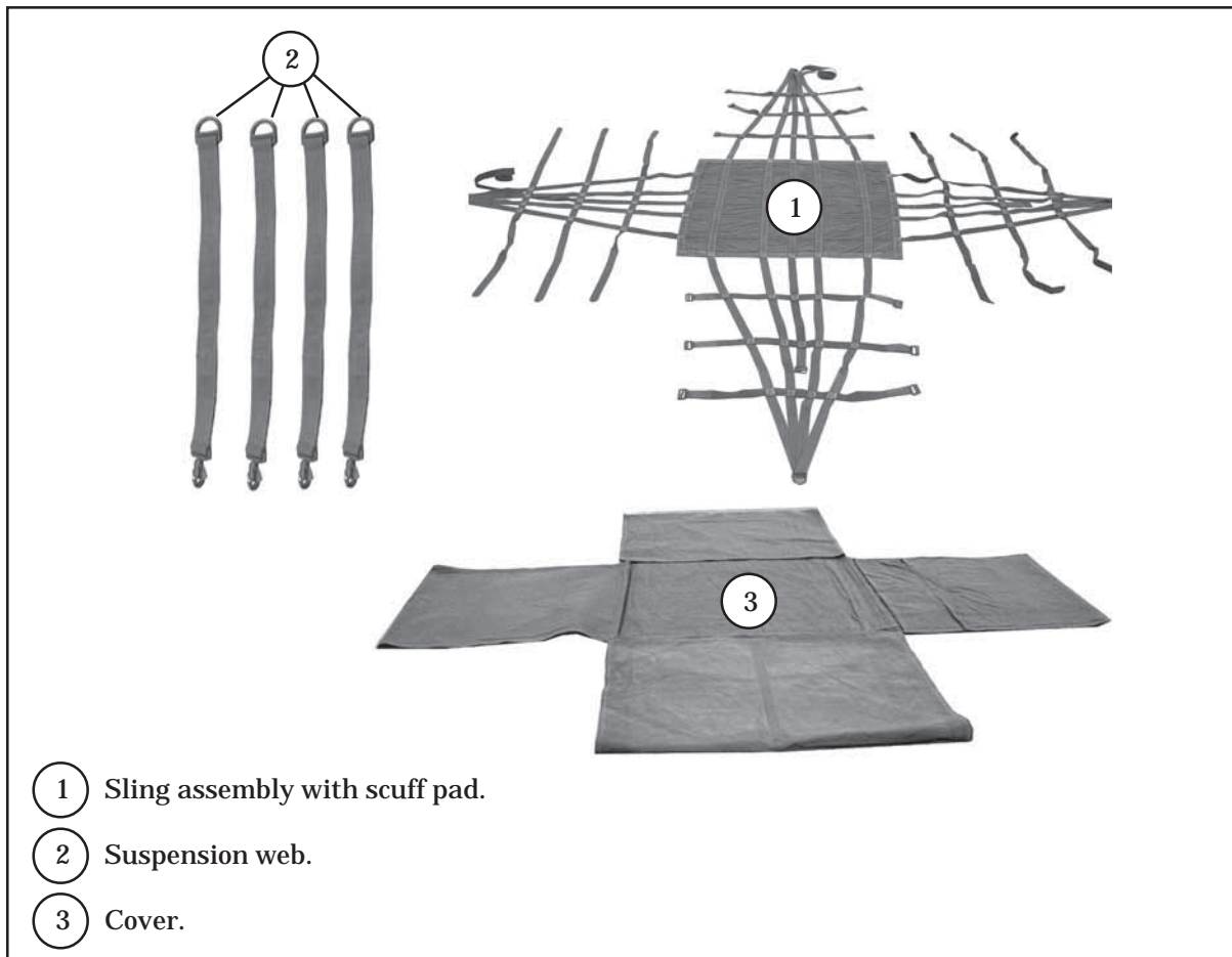
Figure 8-1. A-22 Cargo Bag
