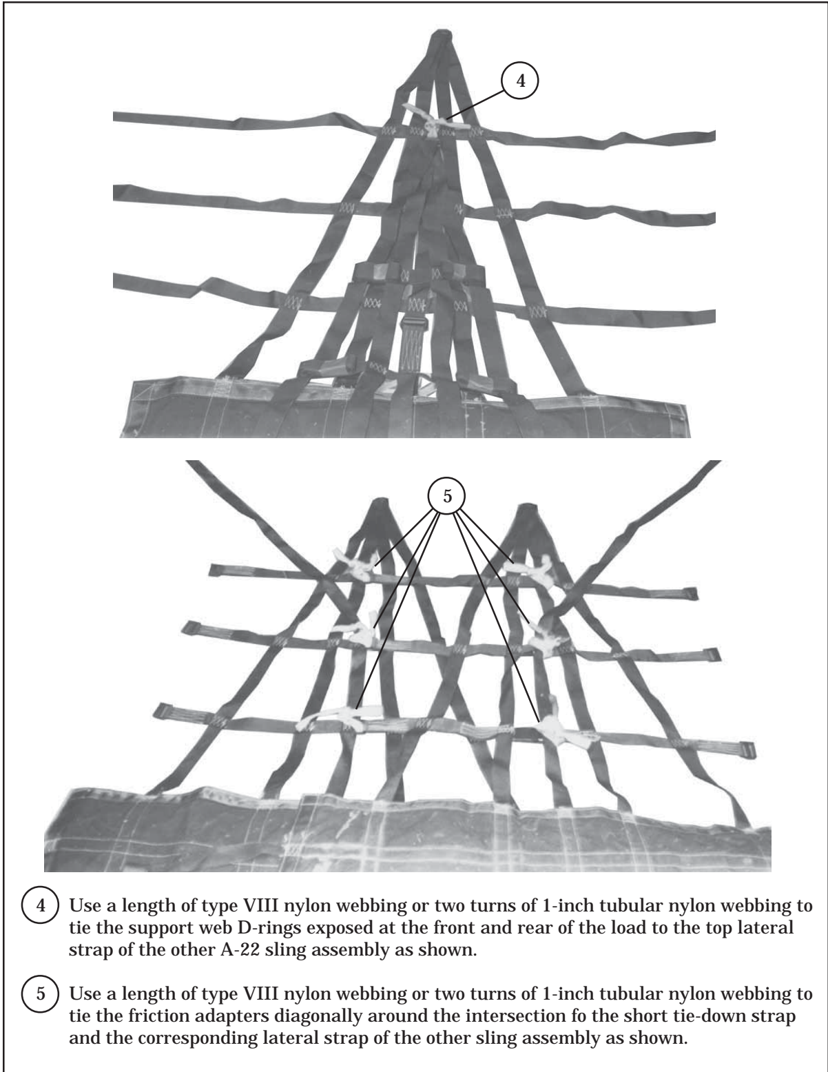
Figure 9-24. A-22 Sling Assemblies Positioned (Continued)
