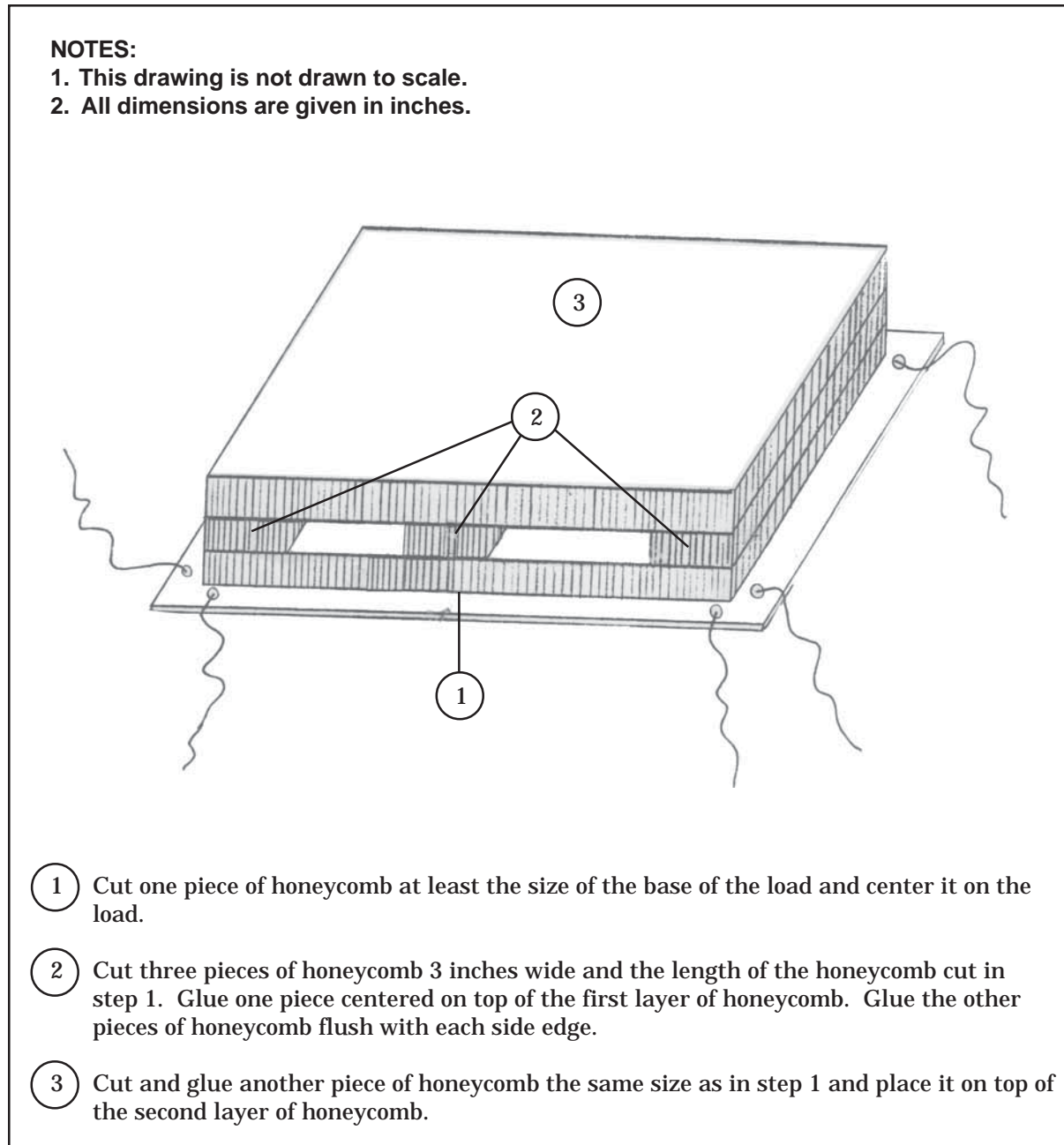
Figure 4-11. Honeycomb Placed
