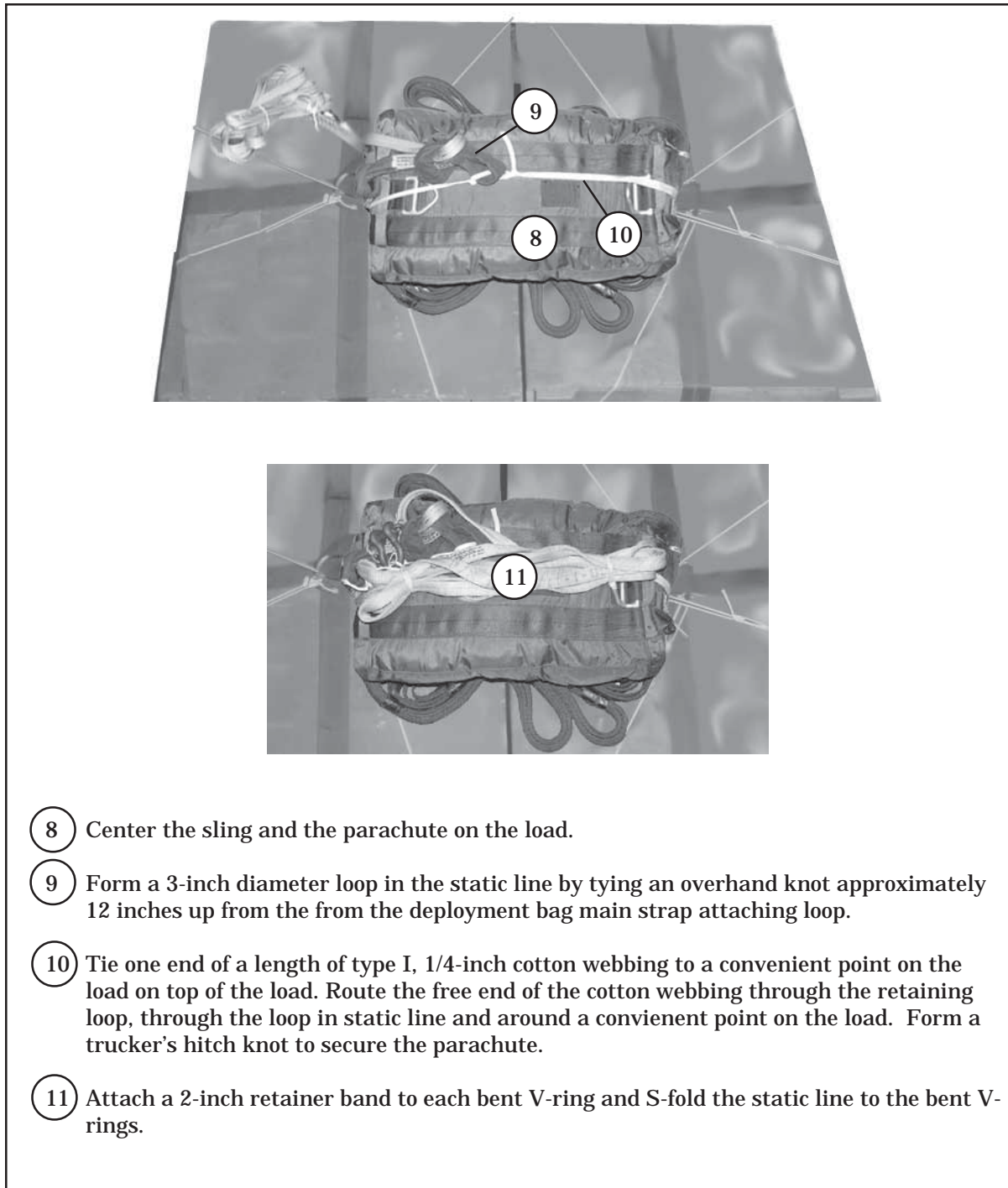
Figure 3-7. One 15-Foot Cargo Extraction Parachute Installed (Continued)
