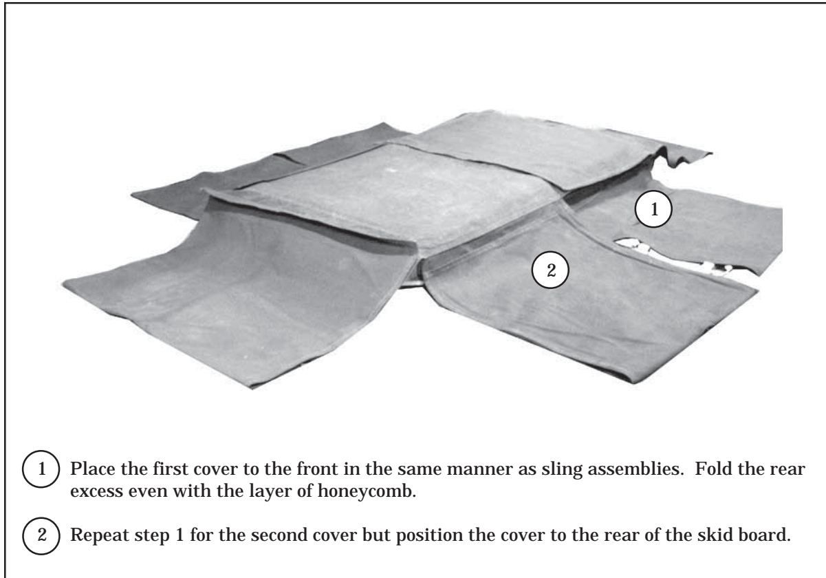
Figure 9-15. Covers Positioned
