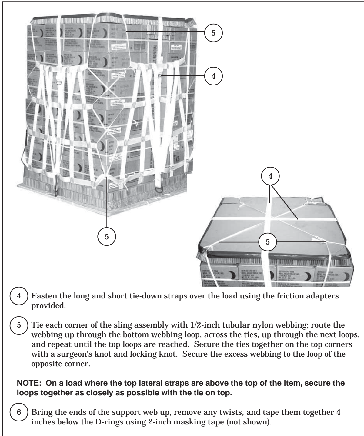
Figure 13-2. Load Positioned and Sling Secured (Continued)
