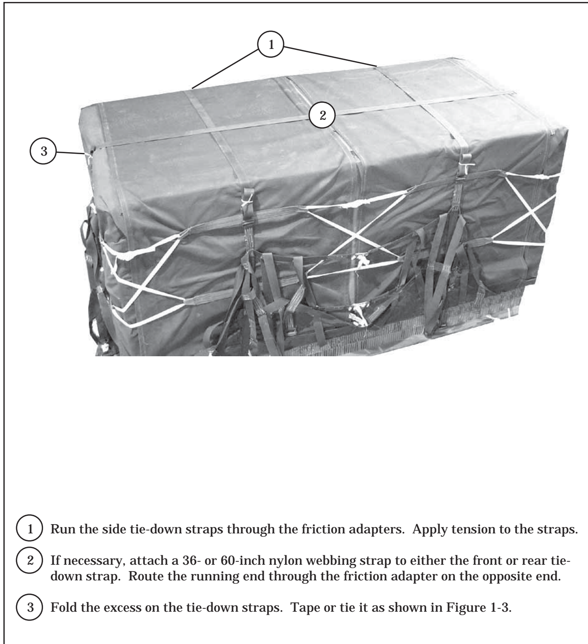
Figure 9-17. Tie-Down Straps Secured
