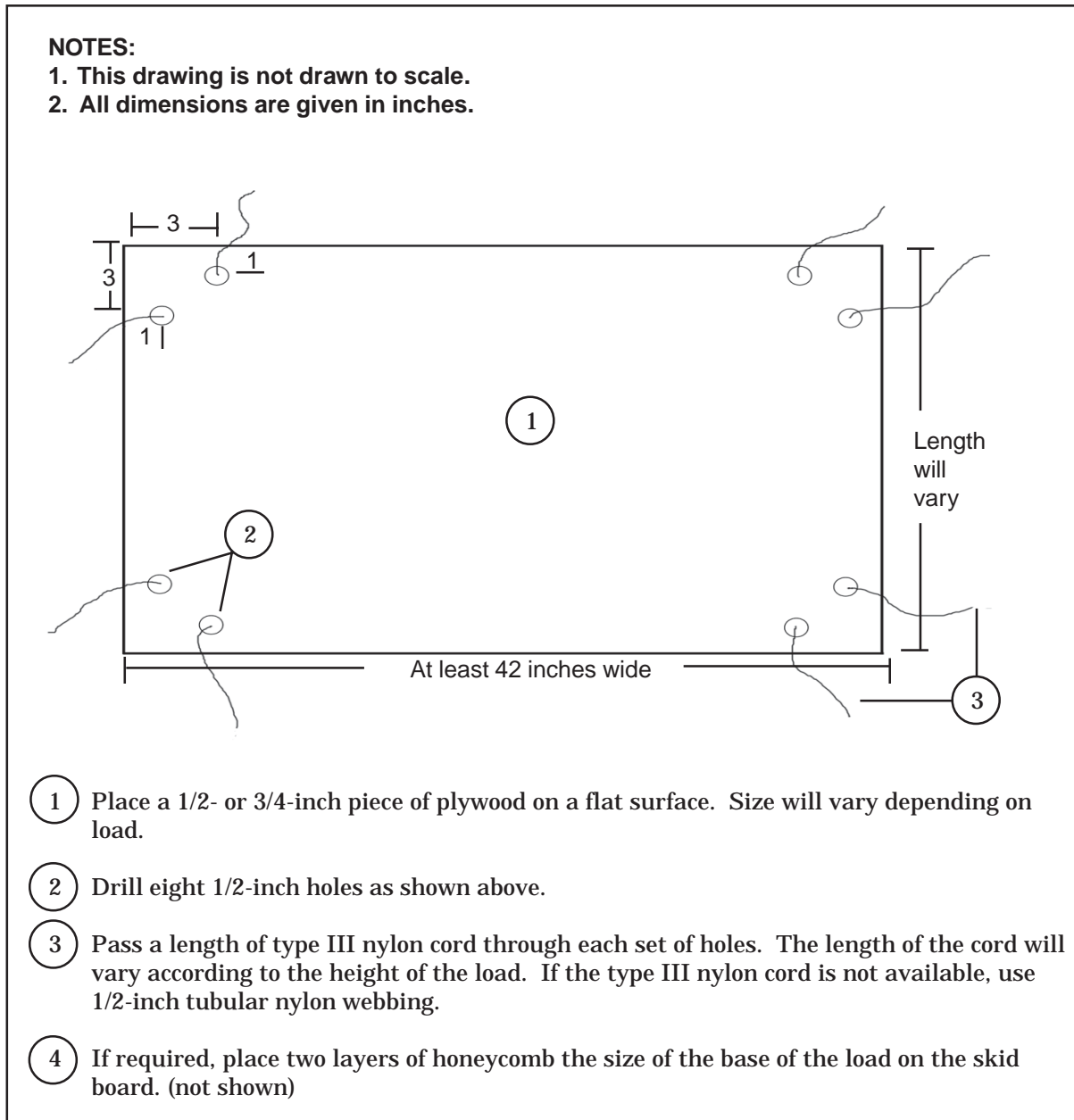
Figure 6-4. Skid Board Prepared
