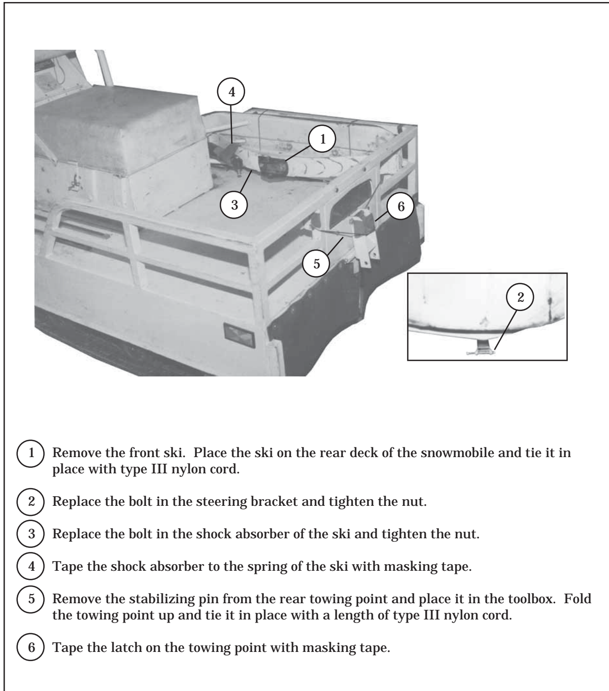
Figure 11-2. Snowmobile Prepared
